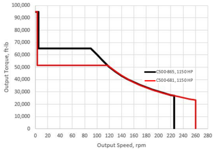
Torque - Speed Curves C500-865 & C500-681
